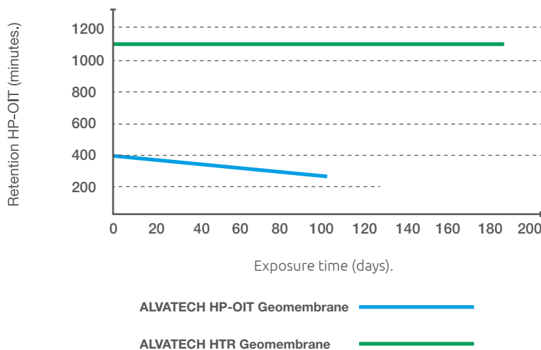
Ageing: HP-OIT retained after 6 months. (ASTM D 5721/5885)
