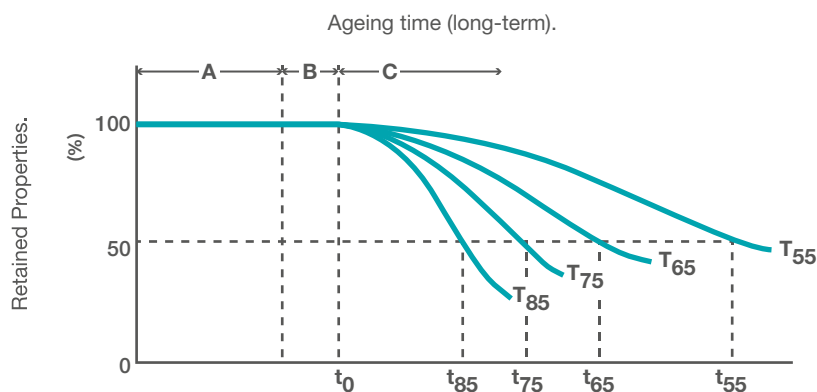
A = Antioxidant depletion time. B = Induction time. C = Time to reach 50% degradation of properties.
