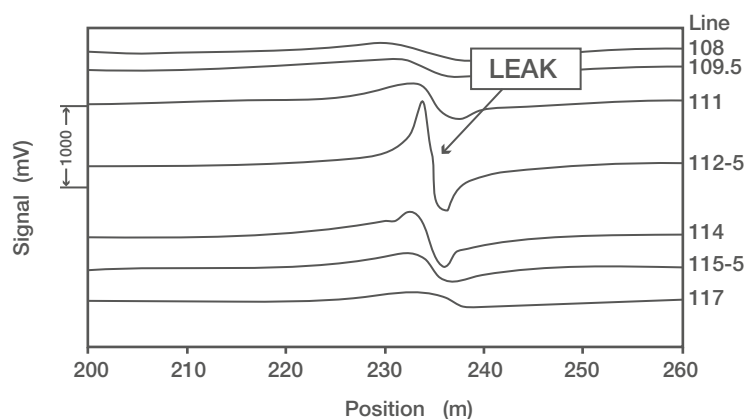
Leak detection graph (Source: TRI Environmental Inc, 2013)
