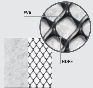
TENAX HF
